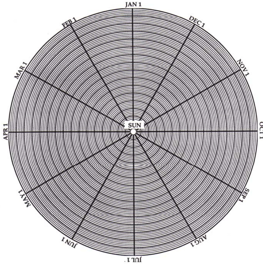
Graph 3.1 EARTH-SUN DISTANCE FOR ONE YEAR The heavy printed circles are separated by 10 million kilometers. The lighter circles are spaced 2 million kilometers apart.
